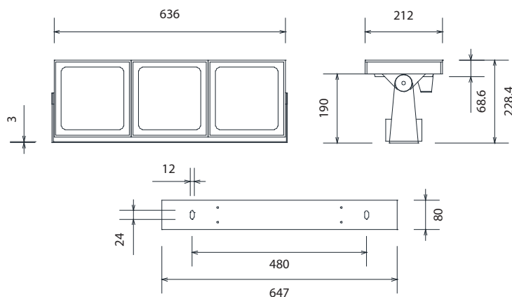
Dimension Drawing (mm)
