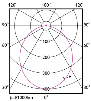
Light Distribution Diagram - 59448 MESON 105 7.5W 30K WH recessed TR
